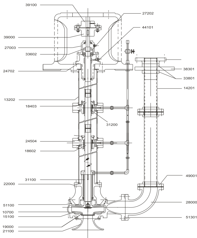
SHS PUMP TYPICAL DRAWING
