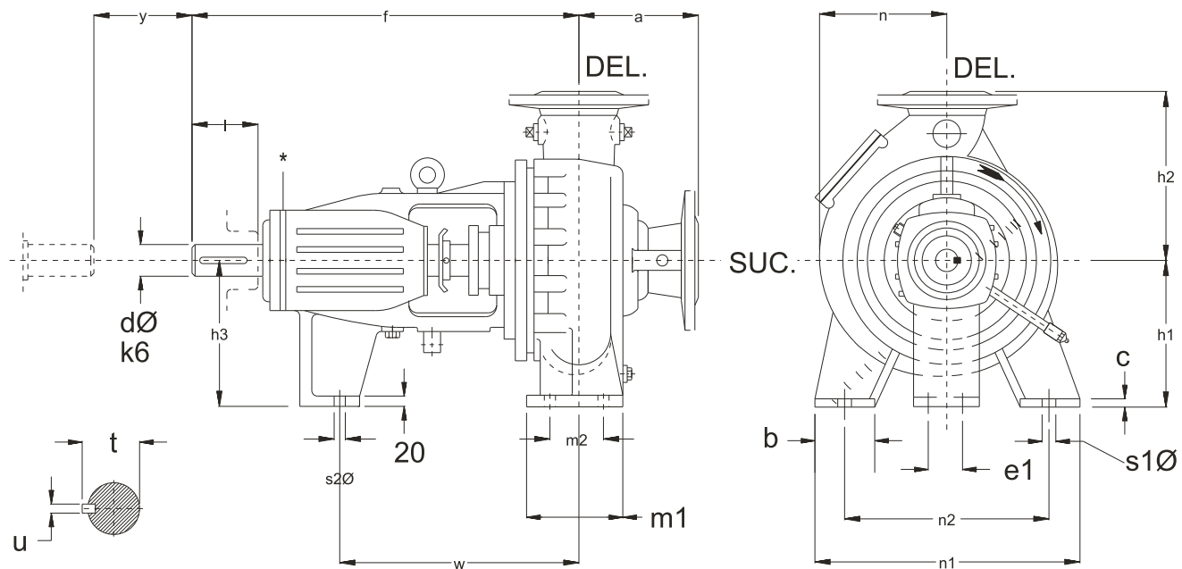
Shaft End
