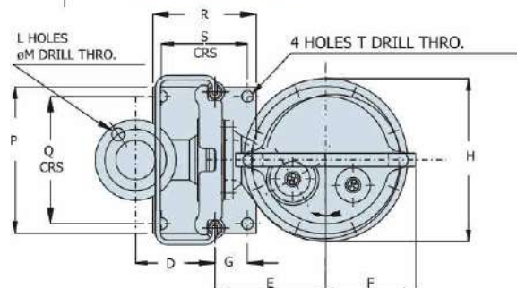
PLAN OF PUMP AND CONNECTOR UNIT ONLY
