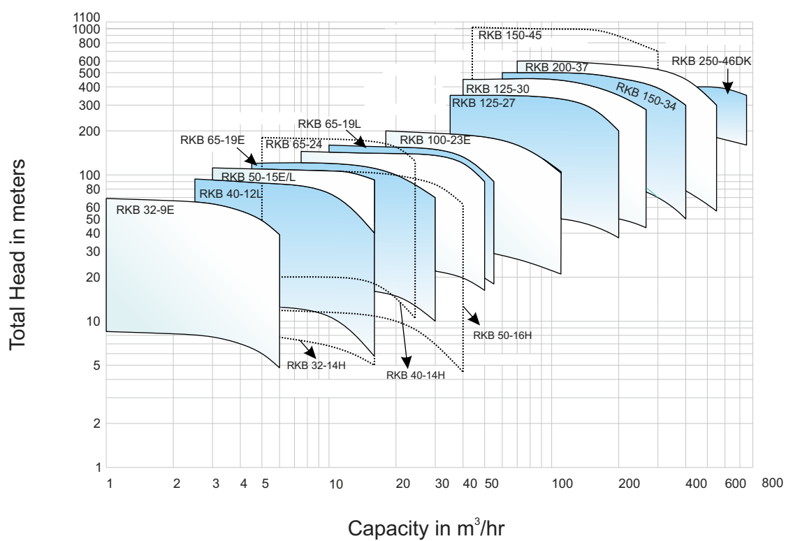
Pump at 2900 rpm-50Hz
